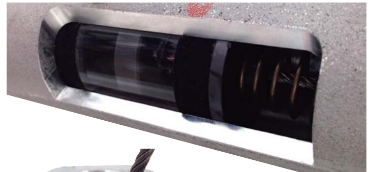
Integrated Liquid Seal cartridge cutaway (above)
